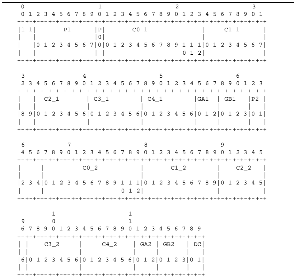
Figure F.3.5/H.225.0 - G.729-12 Packetization Format for the Backward Adaptive Mode
