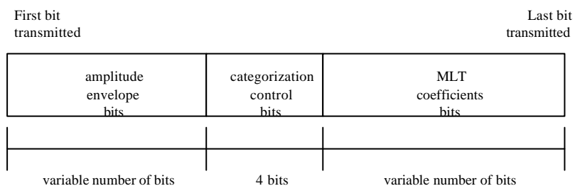
Figure F.6.1/H.225.0 - G.722.1 Major Bitstream Fields and their Order of Transmission
