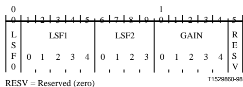
Figure F.3.1/H.225.0 – Annexes B/G.729 F/G.729 and G/G.729 CNG Packetization Format
