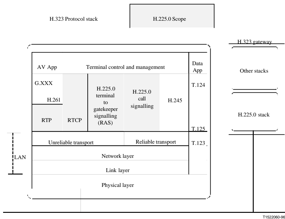
Figure 1/H.225.0 – H.225.0 Scope
