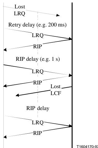
Figure 2/H.225.0 – Example Use of RIP message
