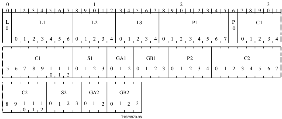
Figure F.3.2/H.225.0 - G.729, Annex A/G.729, and Annex C/G.729 Packetization Format
