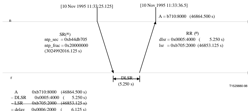
Figure A.2/H.225.0 – Example for round-trip time computation
